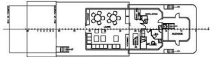
BRIDGE DECK
