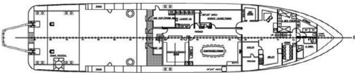
MAIN DECK
