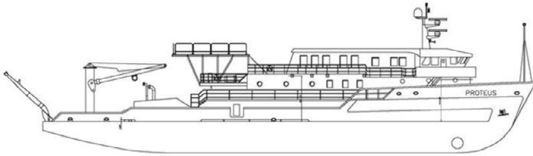
STARBOARD SIDE SCALE 1/8" = 1'-0"
