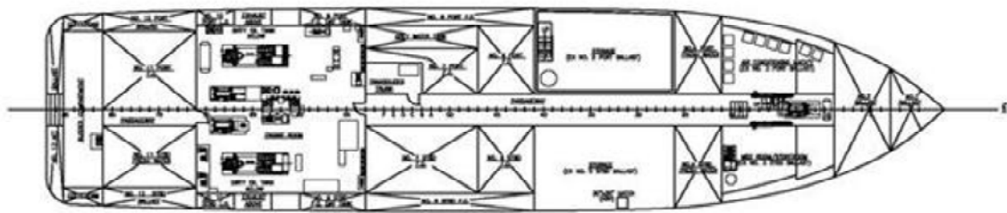
HOLD PLAN
